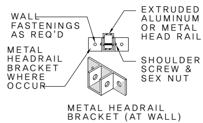
PILASTER / DETAIL
