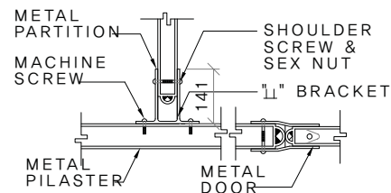
PIN/PILASTER / DETAIL
