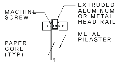
PILASTER / RAIL DETAIL
