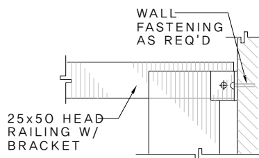
PILASTER / RAIL DETAIL
